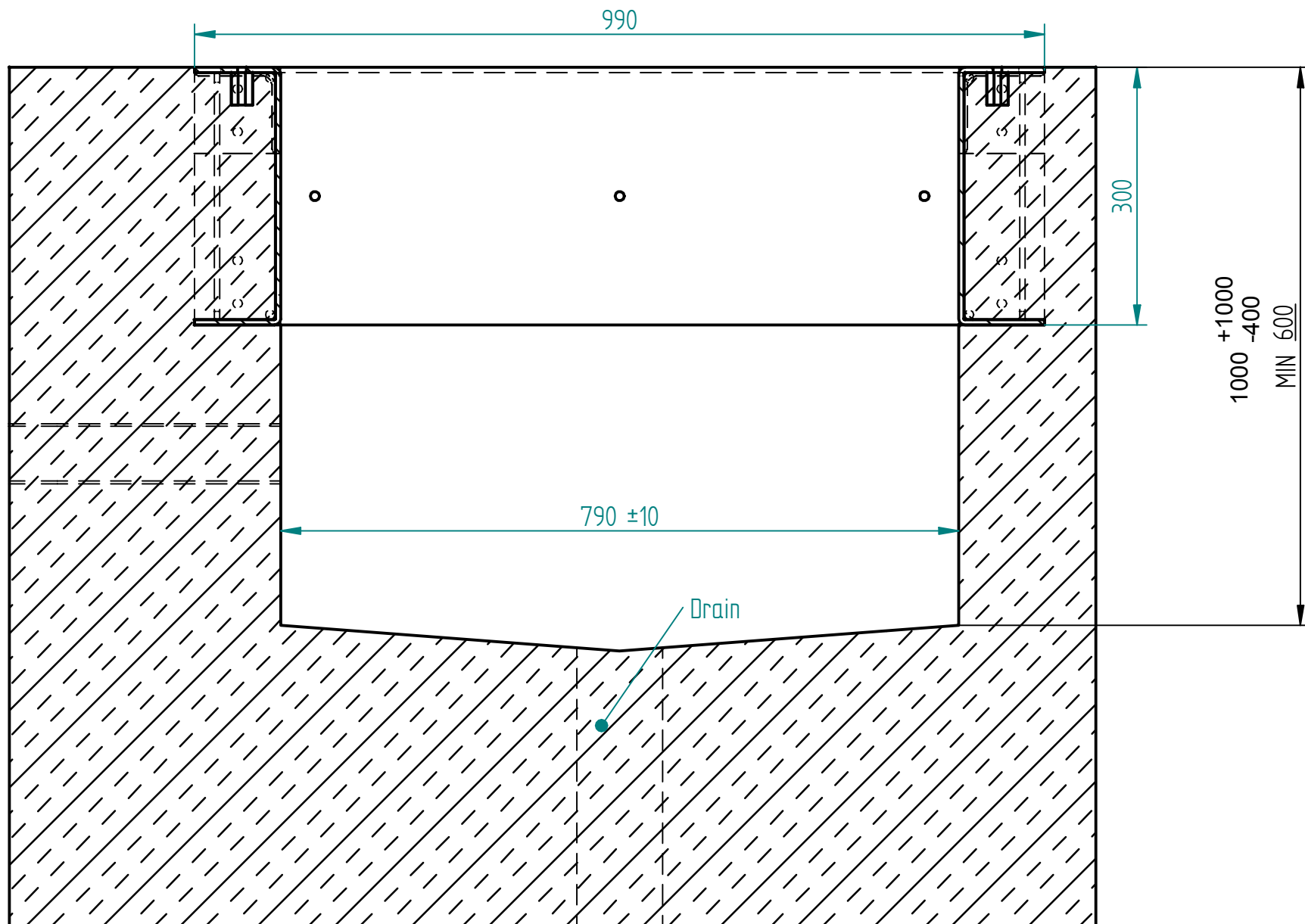
SECTION E-E
